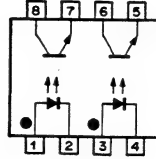
PC627 (SHARP) TTL-PHOTOELECTRIC CELL — TOP VIEW —
